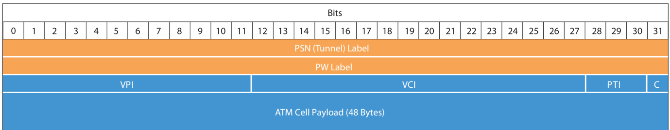
Figure 9. N-to-one encapsulation with two MPLS labels
