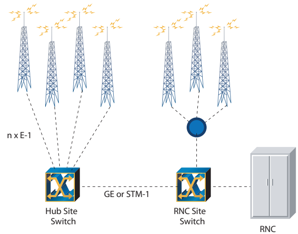
Figure 16. Queuing delay in Hub Site Switch
