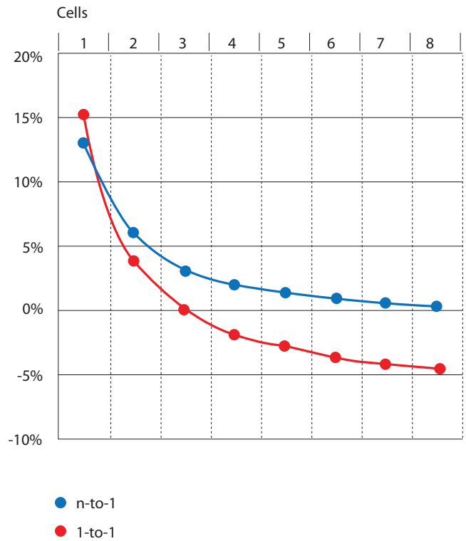
Figure 12. Bandwidth efficiency of ATM pseudowires
