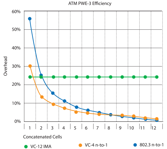
Figure 14. Overhead of ATM PWE3 on Ethernet, VC-4 and ATM IMA on VC-12 compared to ATM on VC-4
