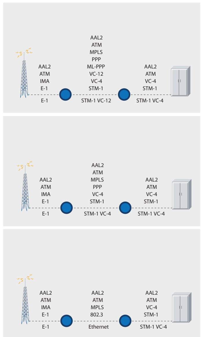
Figure 7. ATM over MPLS via pseudowires
