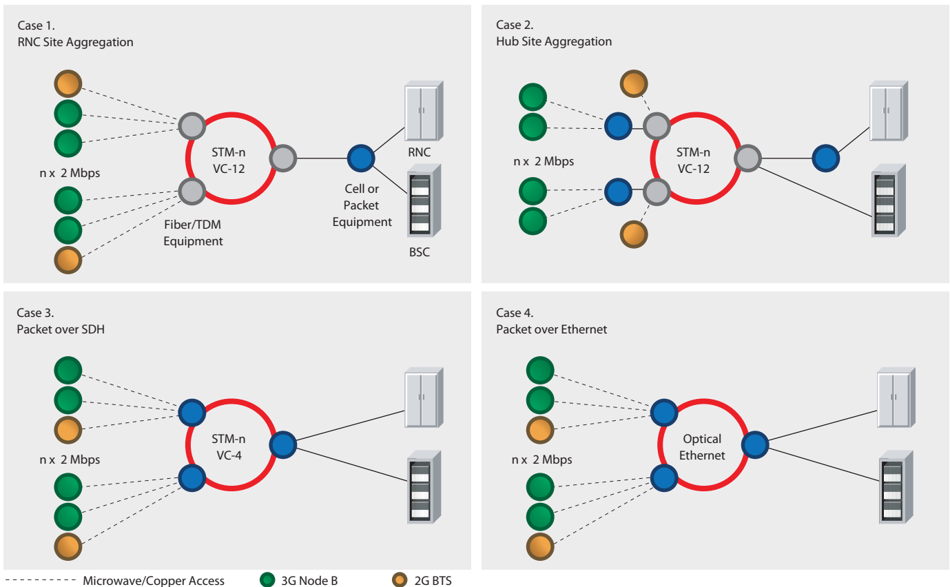
Figure 3. RAN evolution scenarios
