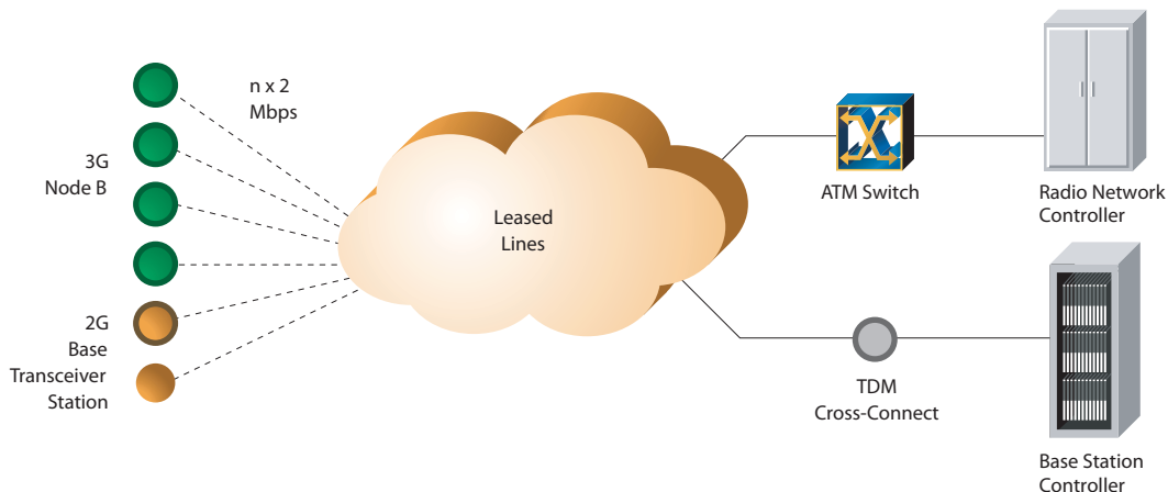
Figure 1. Leased line and microwave radio transport in 2G and 3G networks
