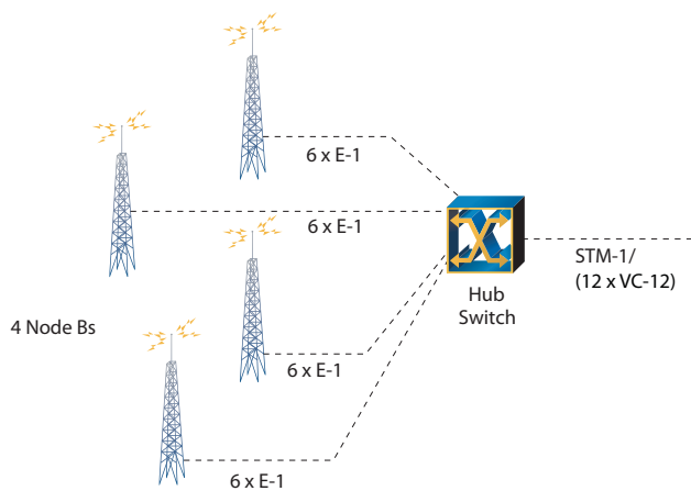
Figure 18. Hub site with STM-1/VC-4 uplink
