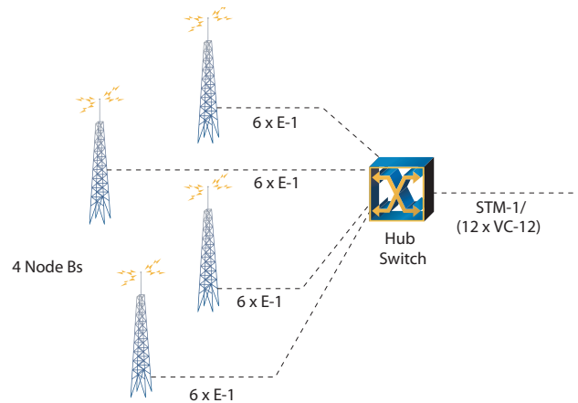
Figure 17. Hub site with STM-1/VC-12 uplink
