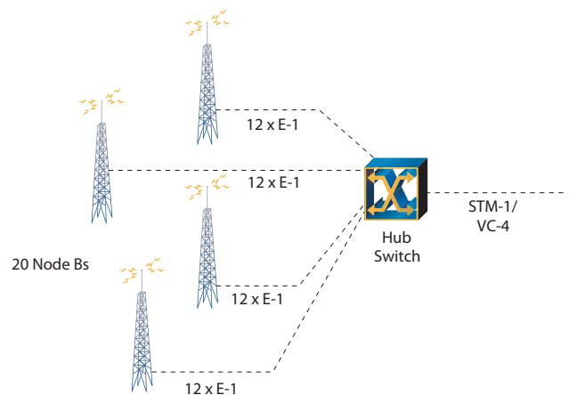
Figure 19. Hub site overbooking scenario
