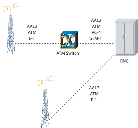
Figure 2. Transport protocol stacks in 3G RAN
