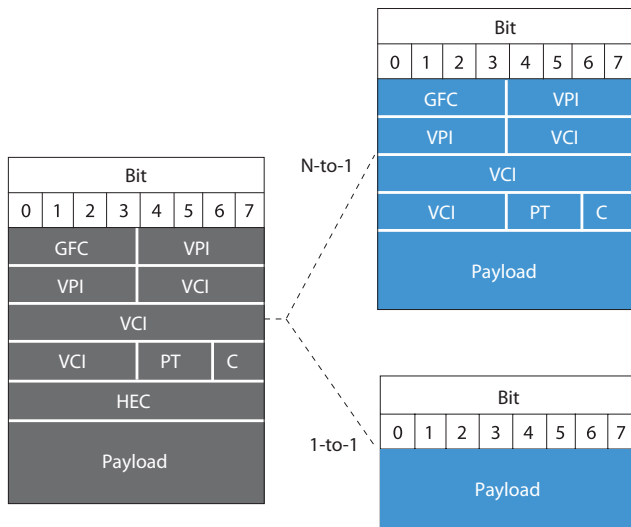
Figure 8. N-to-one and one-to-one ATM cell encapsulation modes
