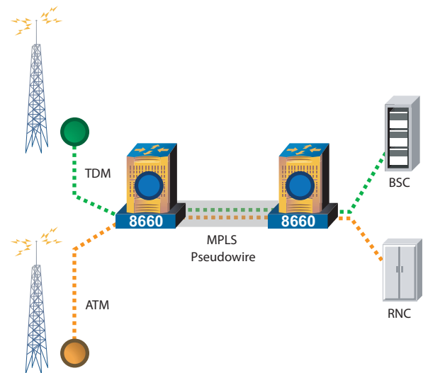
Figure 4. TDM and ATM over MPLS pseudowire
