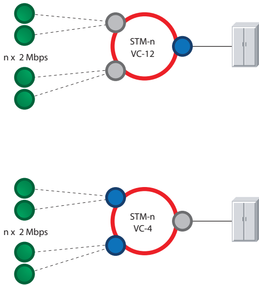
Figure 5. ATM switching at RNC site or remote hub site
