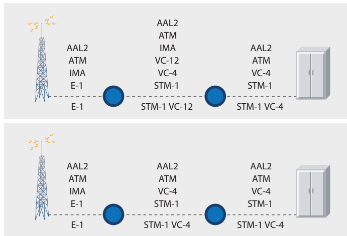
Figure 6. ATM transport and protocol stack alternatives
