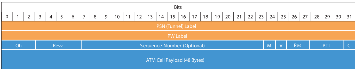
Figure 10. One-to-one encapsulation with three MPLS labels
