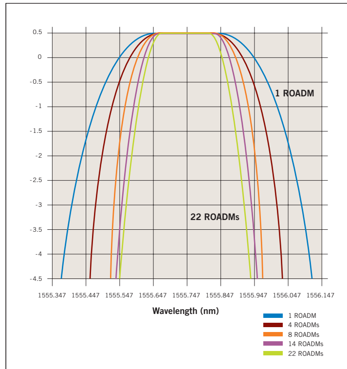
Figure 6. Filter narrowing with increased node count
