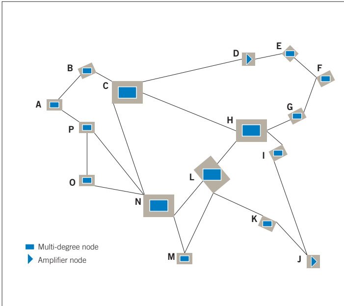
Figure 3. Multi-degree ROADM-based network
