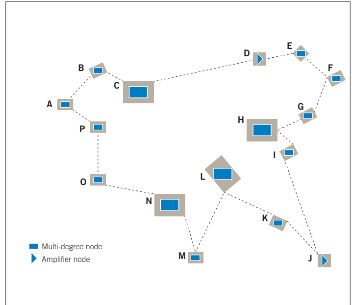
Figure 4. Outer lightpath
