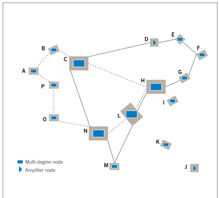
Figure 2. Virtual rings overlaid on optical dynamic core infrastructure
