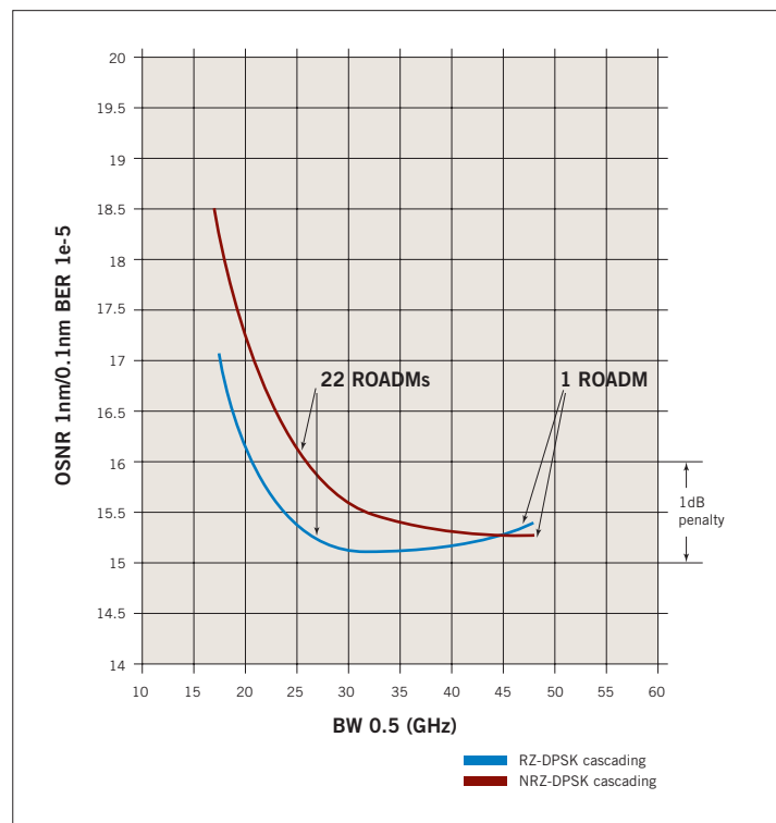
Figure 7. 40 Gbps performances versus ROADM node count
