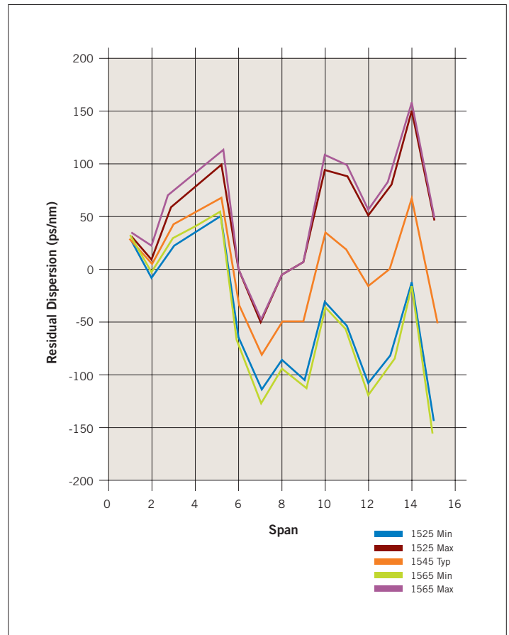
Figure 5. Chromatic dispersion map and walk off for large outer ring
