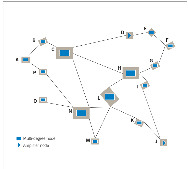
Figure 1. Multi-degree ROADM-based network
