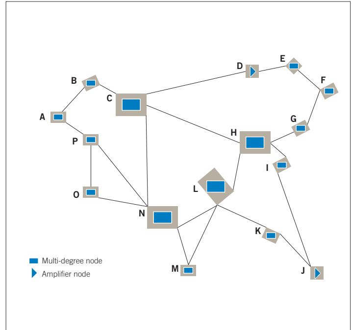
Figure 8. Multi-degree ROADM-based network
