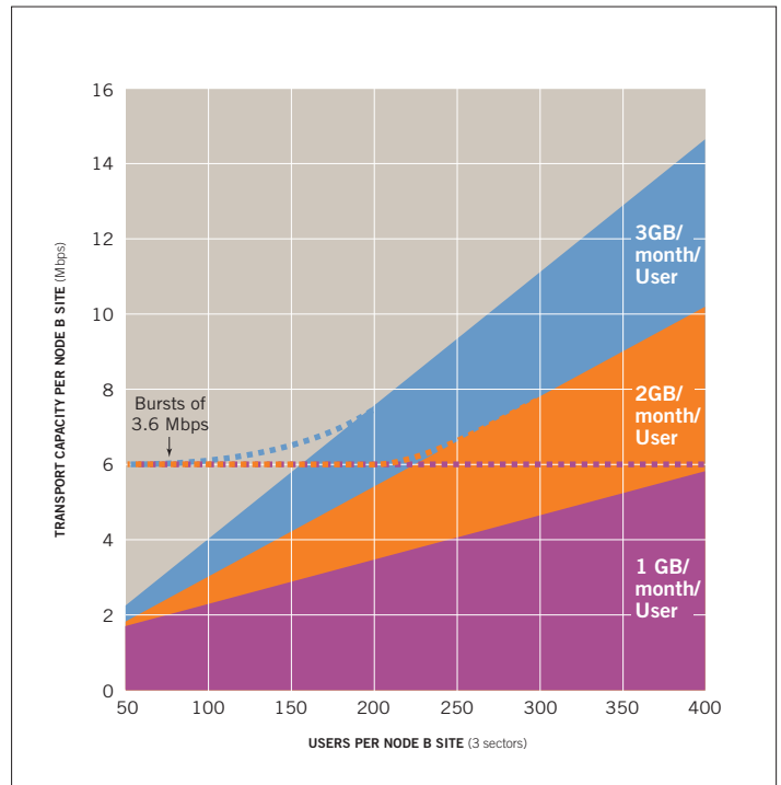
Figure 4. HSDPA backhaul requirements (Source: Tellabs modelling)
