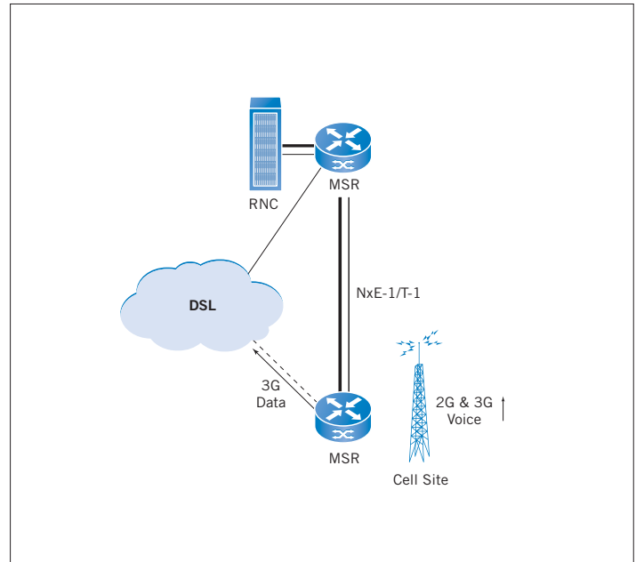
Figure 10. Hybrid DSL with E-1/T-1 leased lines
