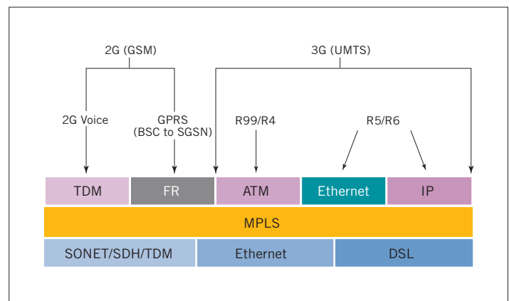
Figure 7. MPLS pseudowires for mobile transport in GSM/UMTS networks
