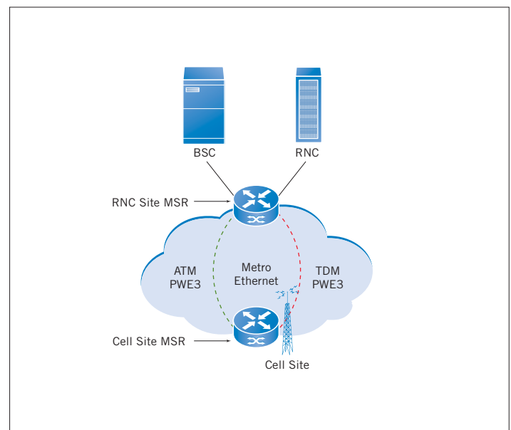
Figure 9. Ethernet to the cell site
