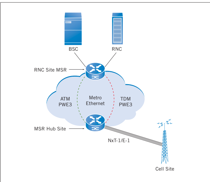
Figure 8. Ethernet to the hub site
